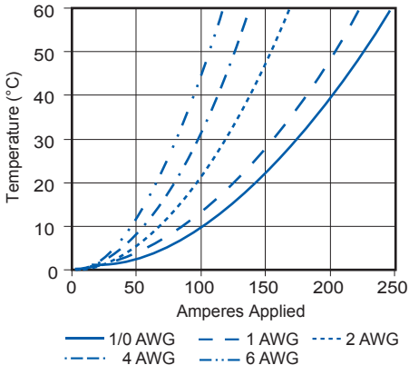
PP120 Singlepole Temperature Rise at Constant Current
