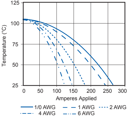
PP120 Multipole Derating vs. Ambient Temperature
