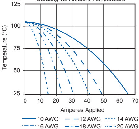
PP15-45 Singlepole Derating vs. Ambient Temperature
