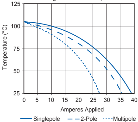
PP25 PCB Derating vs. Ambient Temperature
