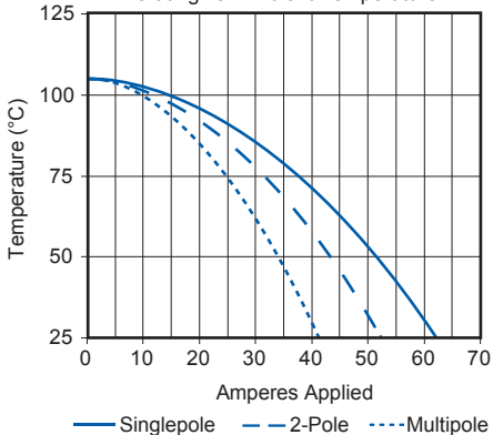
PP45 PCB Derating vs. Ambient Temperature
