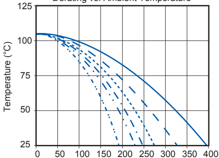
PP180 Multipole Derating vs. Ambient Temperature
