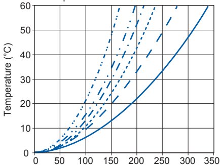
PP180 Multipole Temperature Rise at Constant Current
