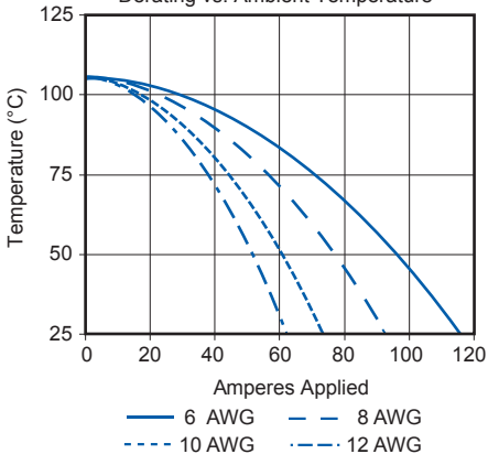
PP75 Singlepole Derating vs. Ambient Temperature
