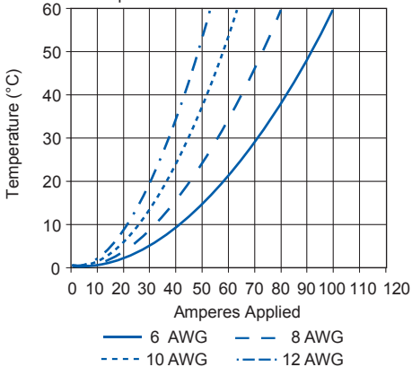
PP75 Singlepole Loose Piece Contact Temperature Rise at Constant Current
