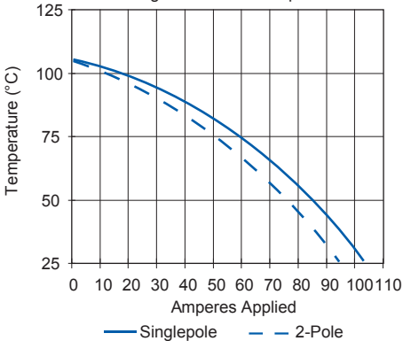
Mini Powerclaw Derating vs. Ambient Temperature
