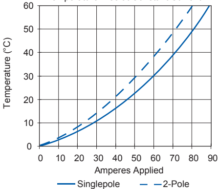
Mini Powerclaw Temperature Rise at Constant Current
