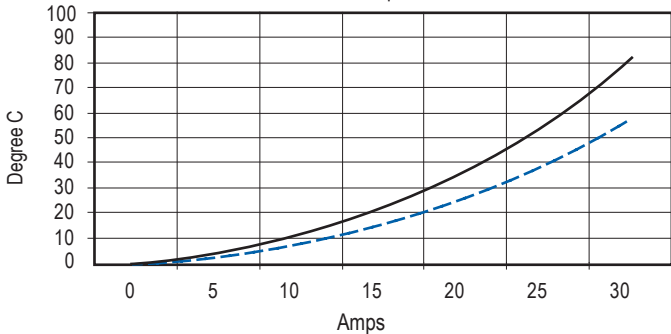
1 Row Current vs Temperature Rise
