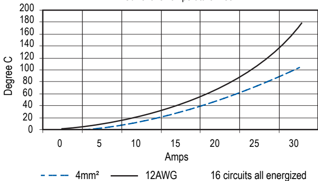
2 Row Current vs Temperature Rise
