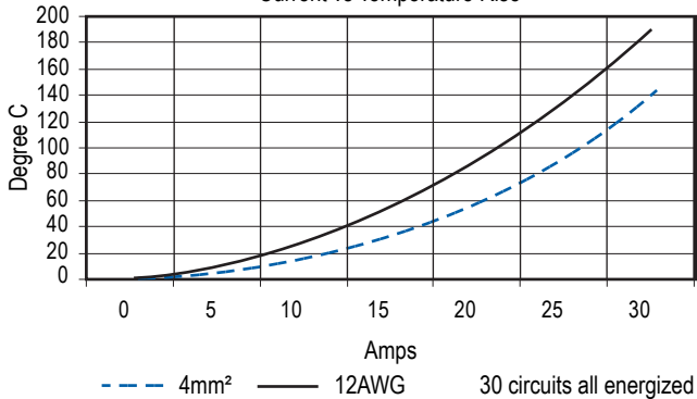
3 Row Current vs Temperature Rise
