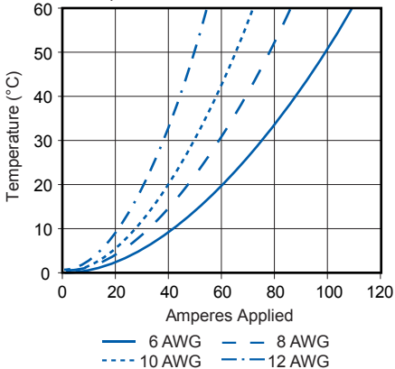
SBS®75G All Contacts Powered Temperature Rise at Constant Current
